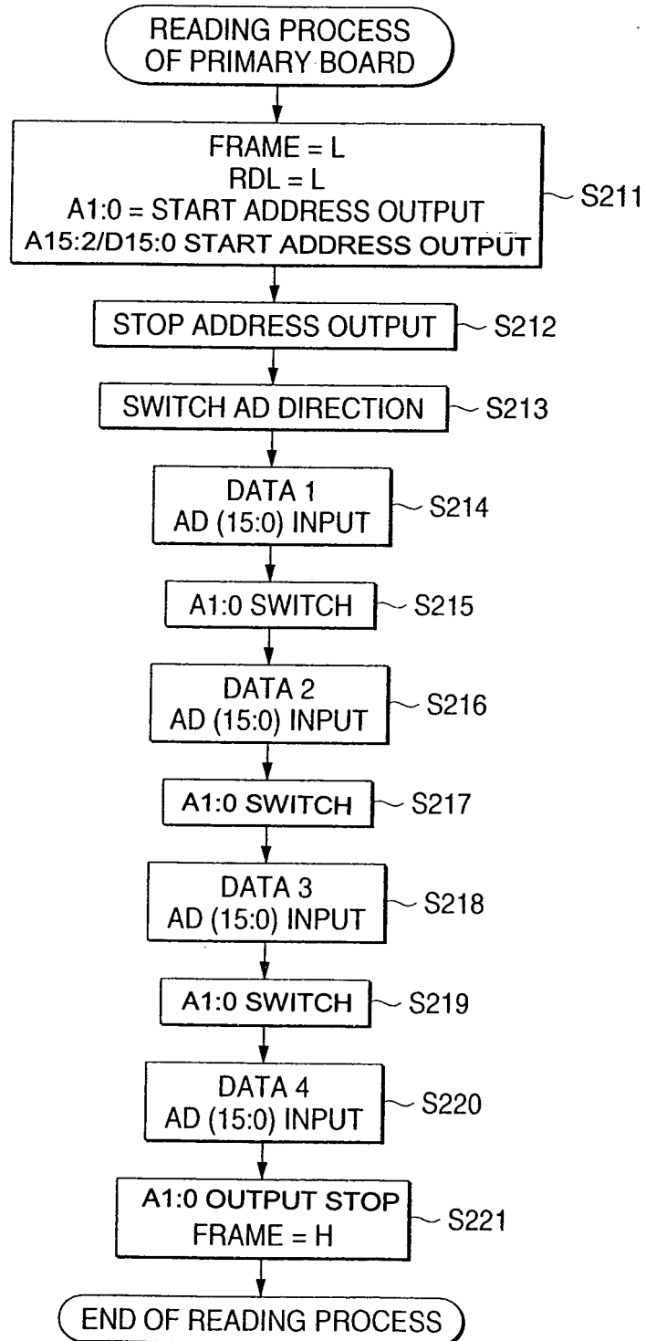
FIG. 20 PRIOR ART
